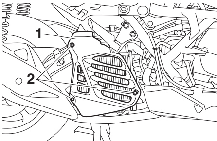
1. Kylarlock 2. Bult
